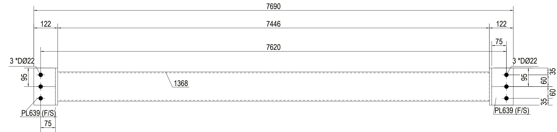
FRONT VIEW
